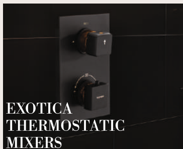
FAUCETS
